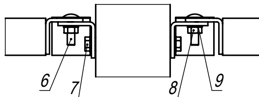
В (1:4)
